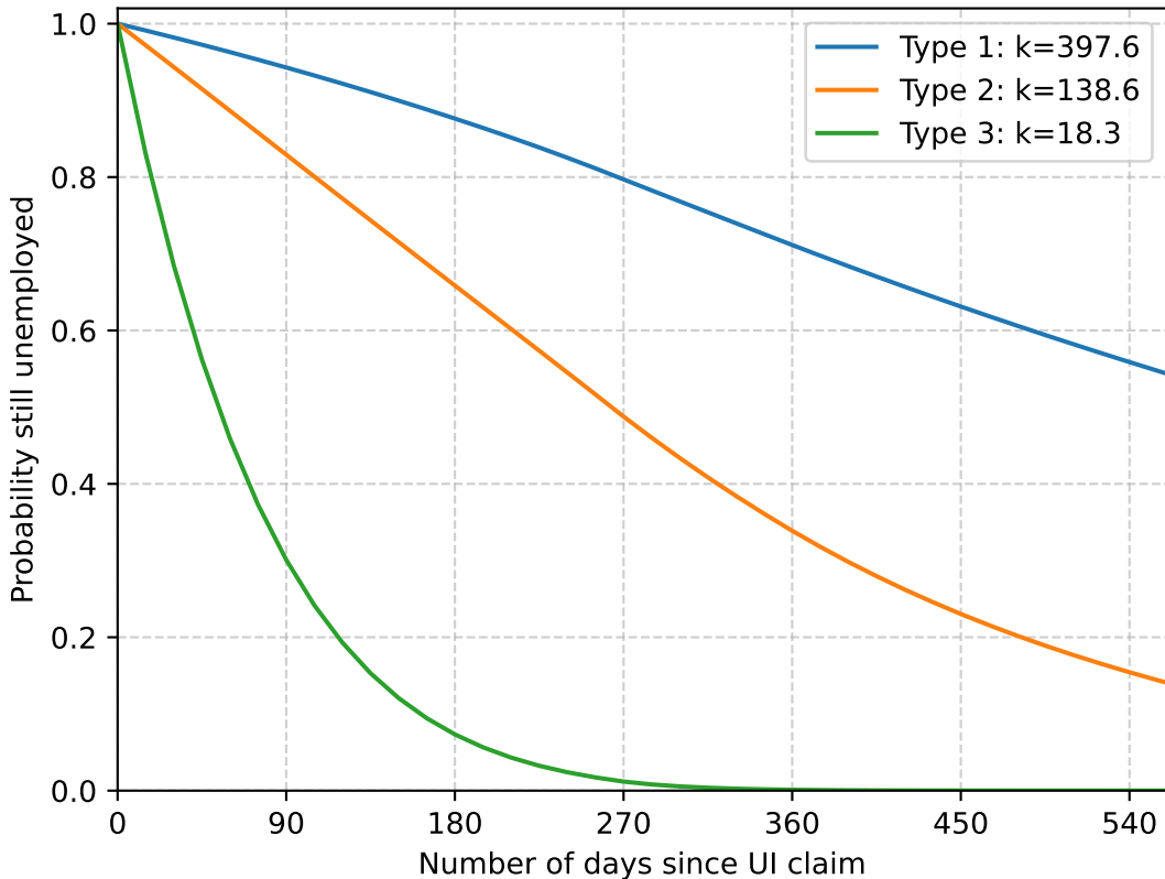
Pre-reform survival by search-cost type
